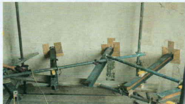
All installed 'I' beams levelled and supported as grout hardens
