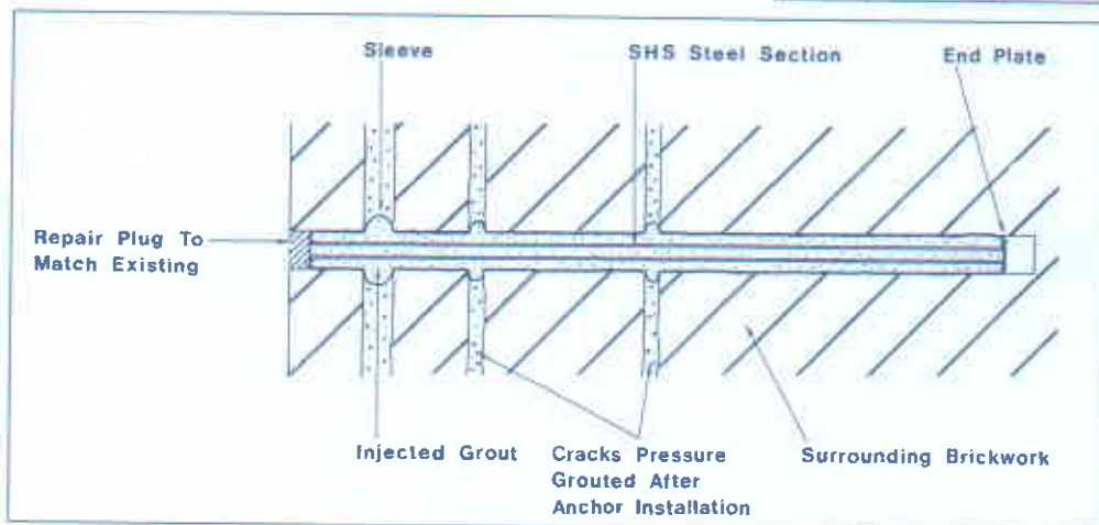
Section through a typical Cintec anchor installation
